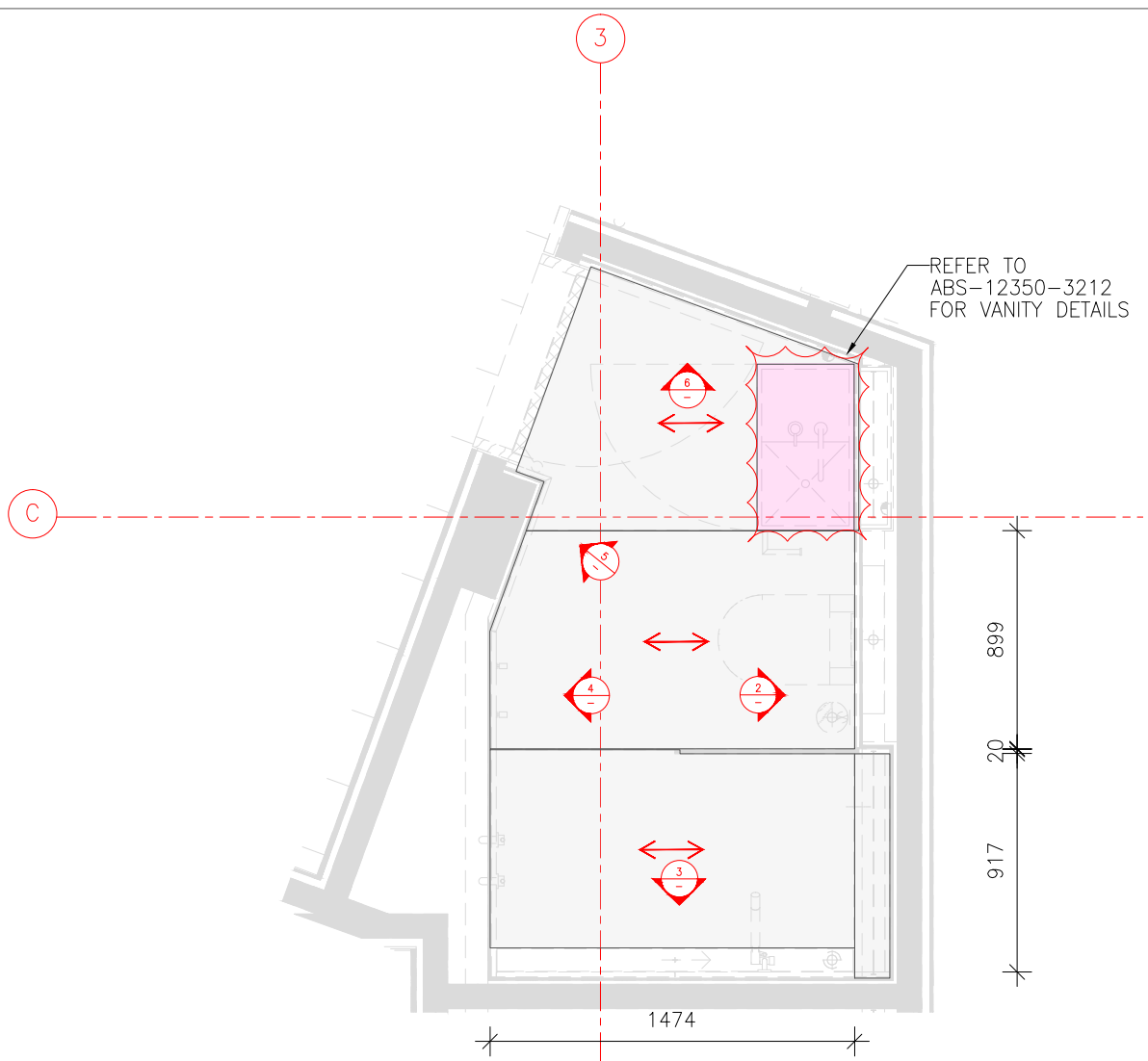
01 GUEST WING-L1 ENSUITE-2 FLOOR PLAN SCALE 1:50 @ A3
