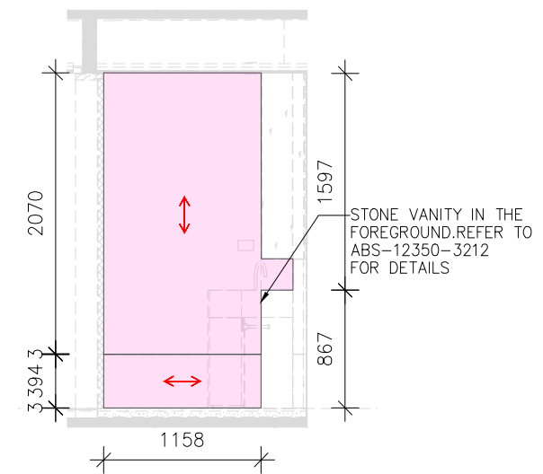
06 ELEVATION-6 SCALE 1:50 @ A3
