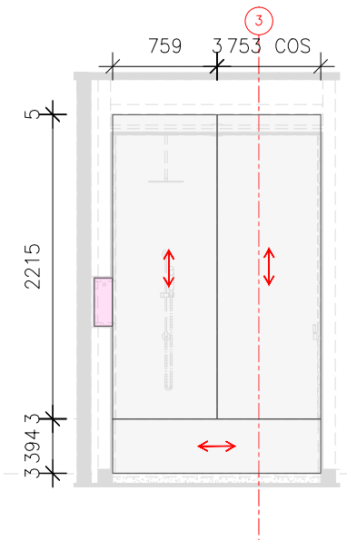
03 ELEVATION-3 SCALE 1:50 @ A3
