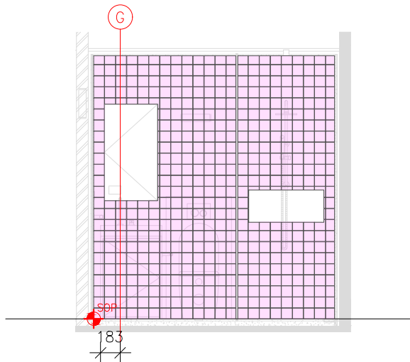
04 ELEVATION-4 SCALE A3 @1:50
