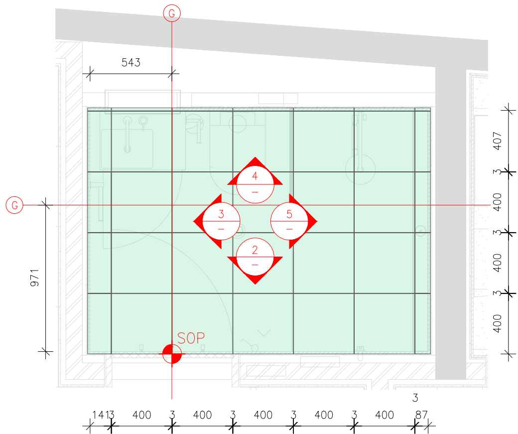
01 GUEST WING-LGF ENSUITE FLOOR PLAN SCALE: A3 @1:25
