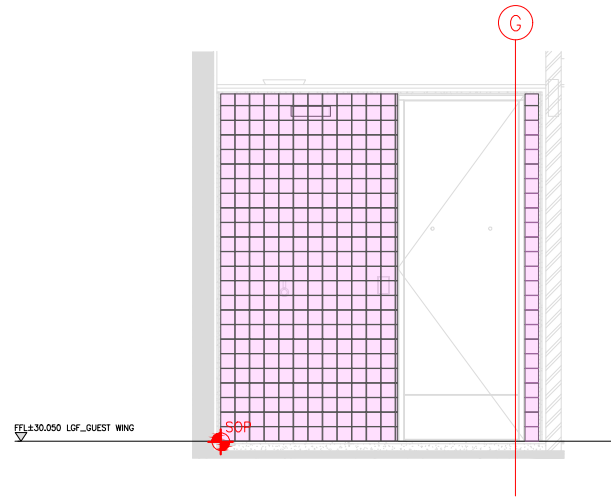
02 ELEVATION-2 SCALE A3 @1:50
