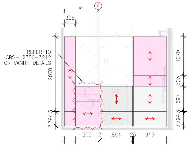
02 ELEVATION-2 SCALE 1:50 @ A3
