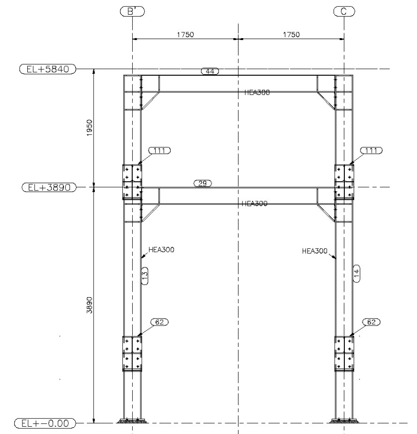
ELEVATION ON 18
