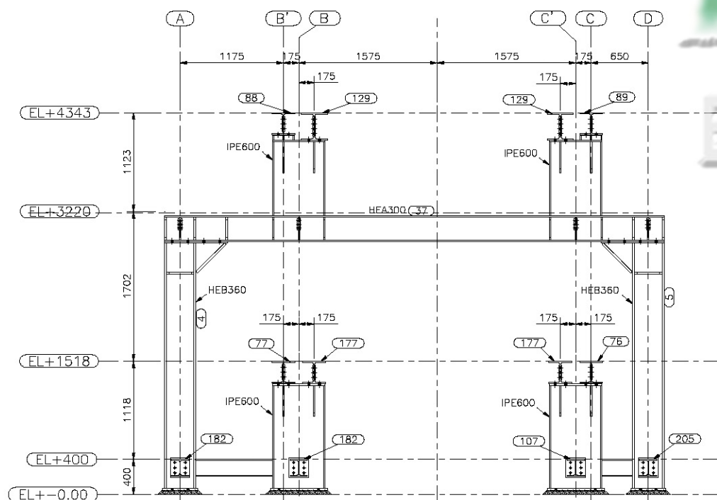
ELEVATION ON 4 TO 15
