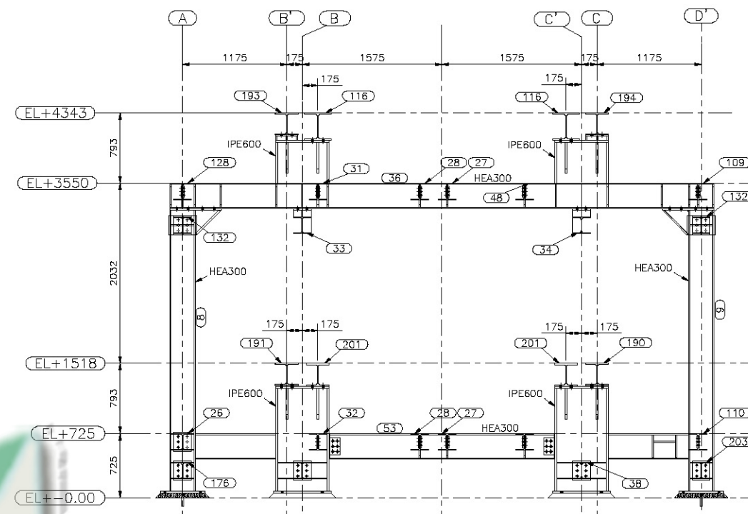
ELEVATION ON 2
