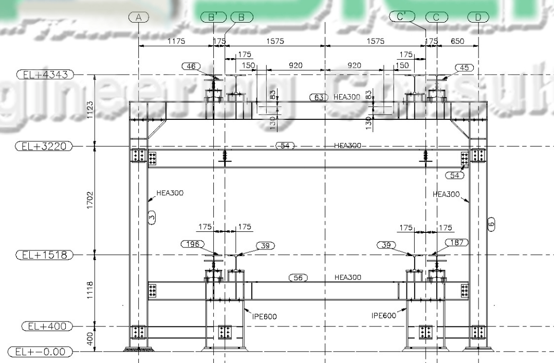
ELEVATION ON 16
