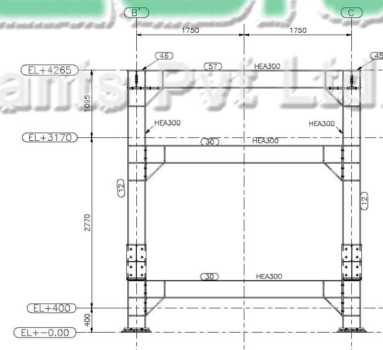
ELEVATION ON 17
