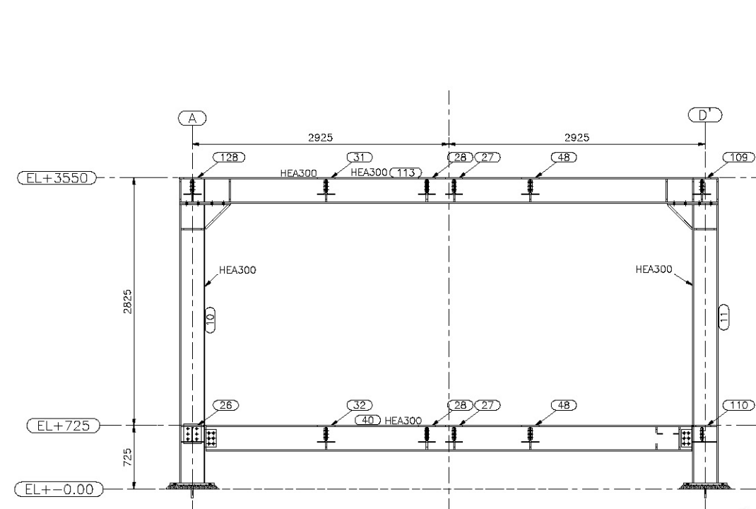
ELEVATION ON 1
